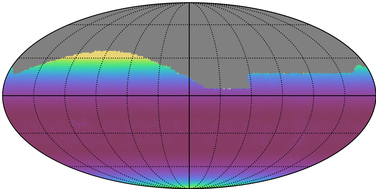
roll_pause_mjdp0_v3.4_10yrs All sky g band: Min airmass
