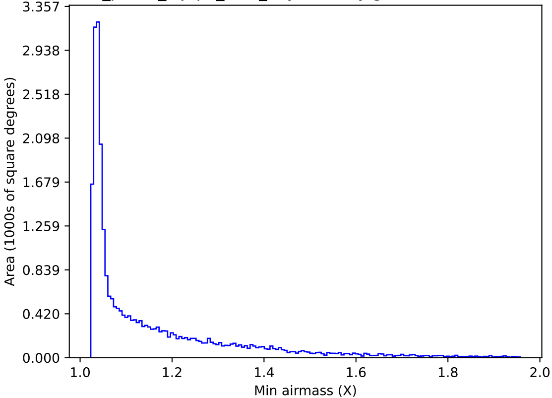
roll_pause_mjdp0_v3.4_10yrs All sky g band: Min airmass
