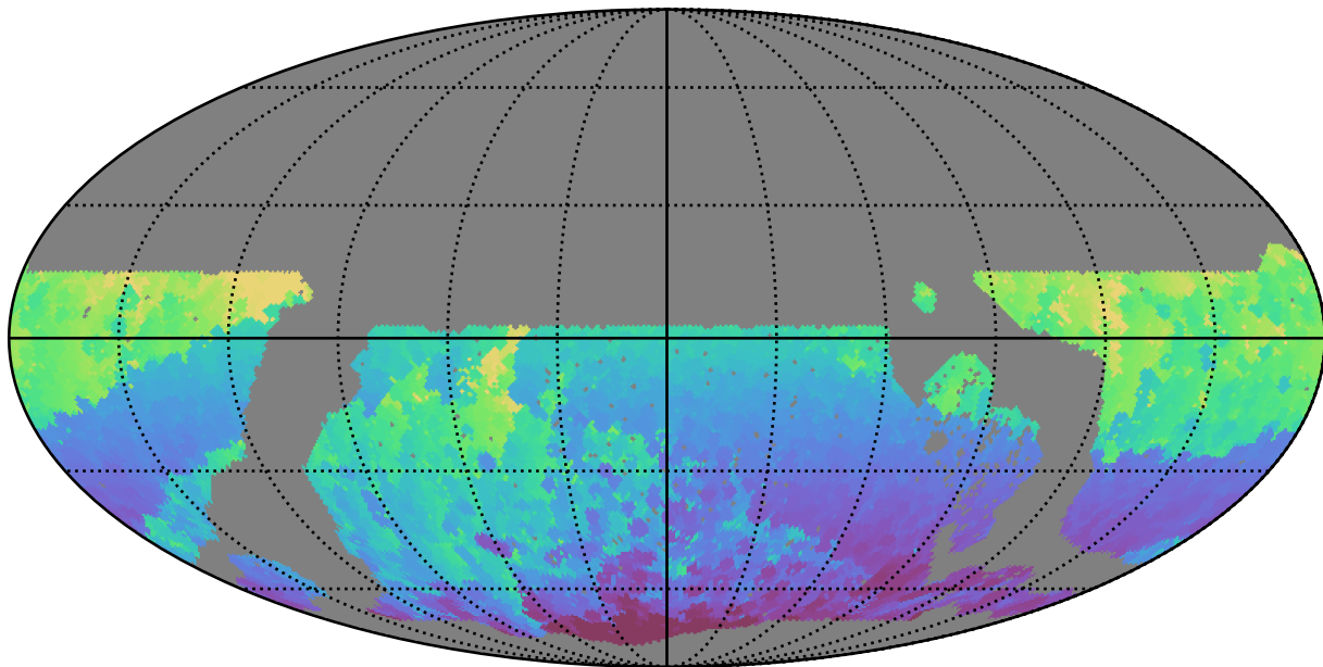
roll_pause_mjdp0_v3.4_10yrs WFD r band: Min HA
