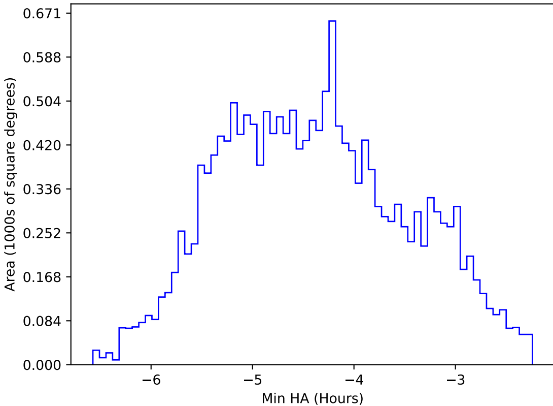
roll_pause_mjdp0_v3.4_10yrs WFD r band: Min HA
