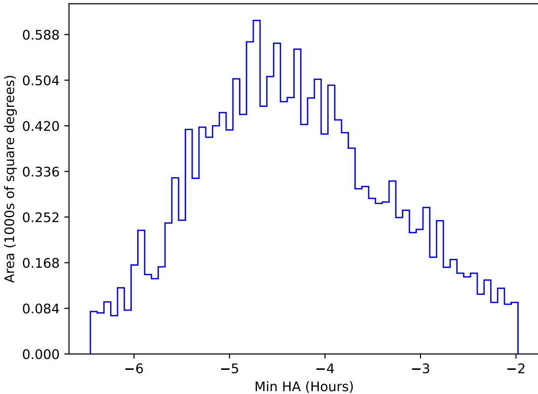
roll_pause_mjdp0_v3.4_10yrs WFD i band: Min HA
