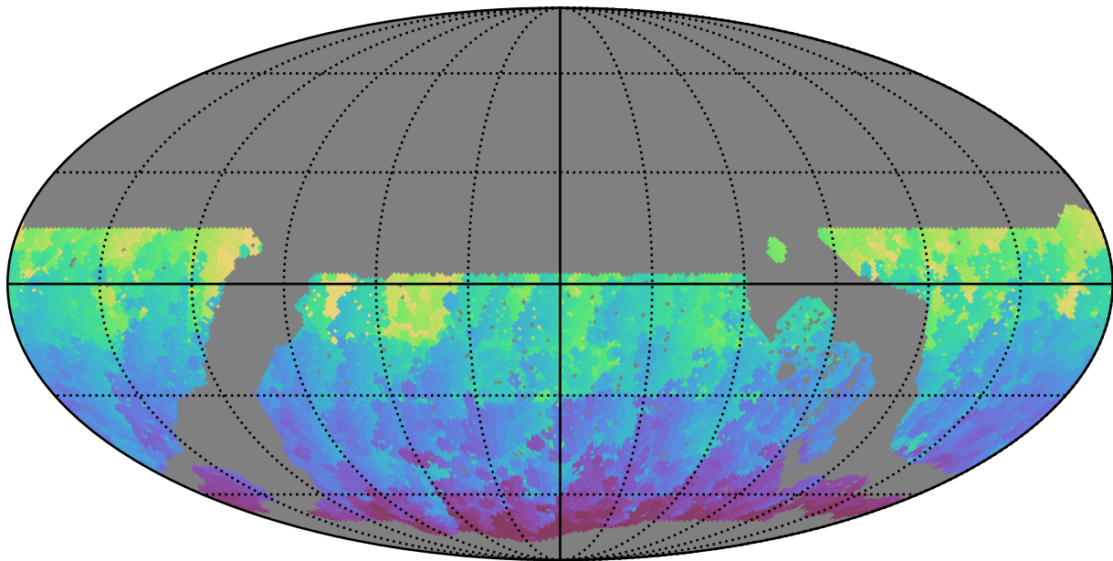
roll_pause_mjdp0_v3.4_10yrs WFD g band: Min HA
