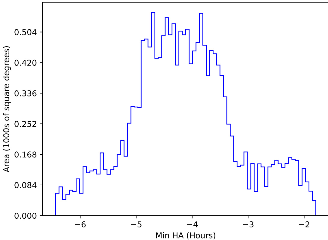
roll_pause_mjdp0_v3.4_10yrs WFD g band: Min HA
