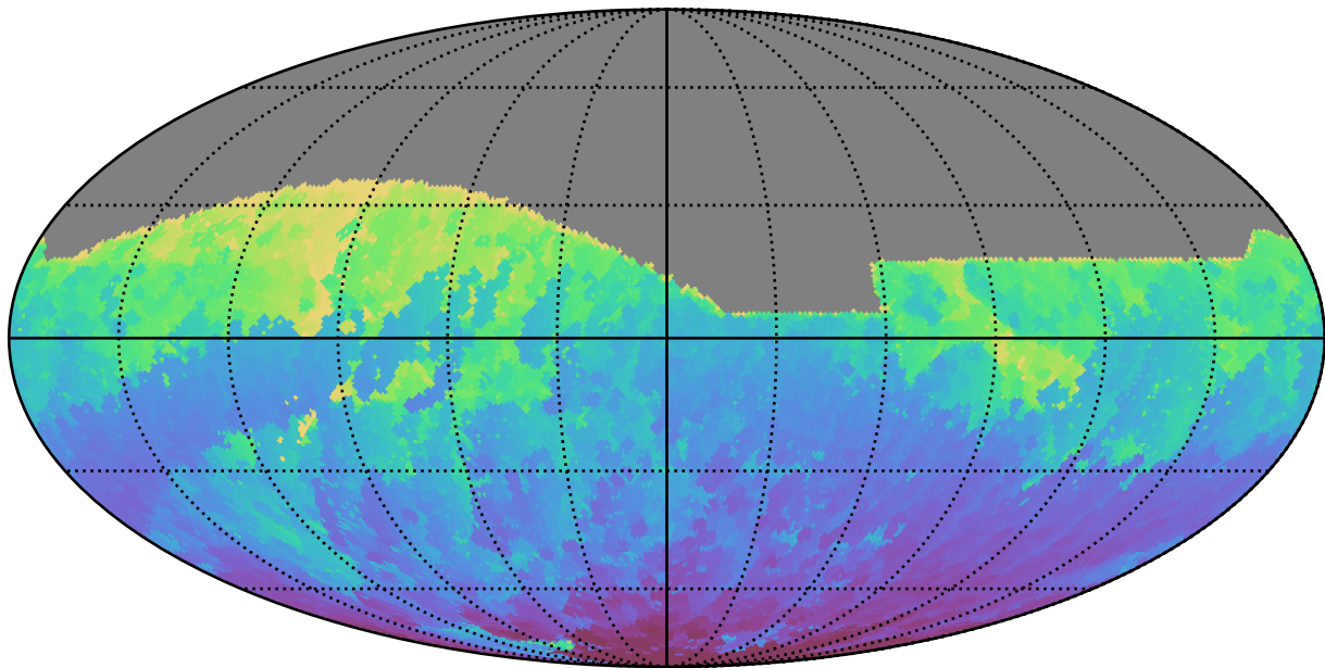
roll_pause_mjdp0_v3.4_10yrs All sky z band: Min HA
