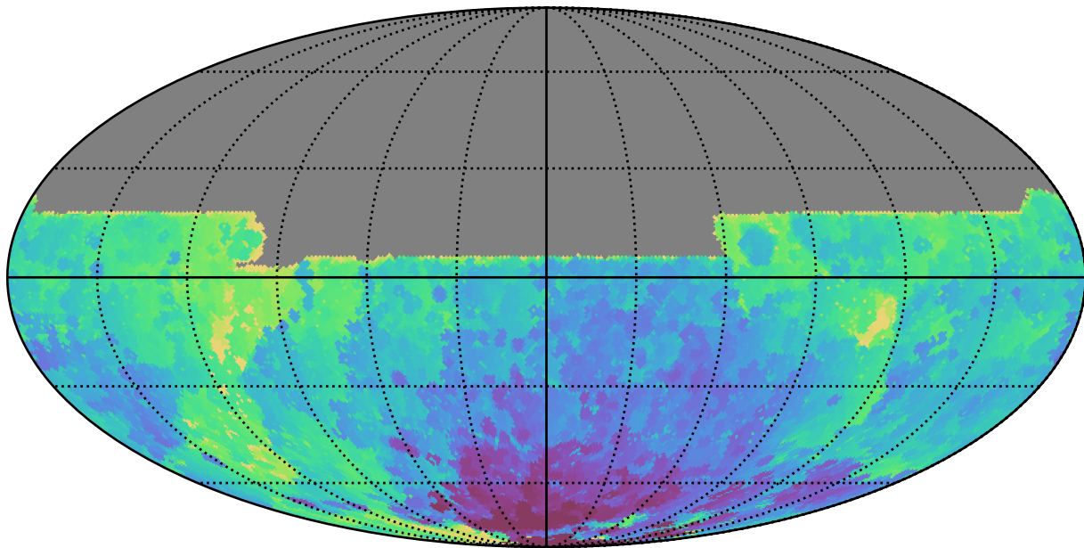
roll_pause_mjdp0_v3.4_10yrs All sky y band: Min HA
