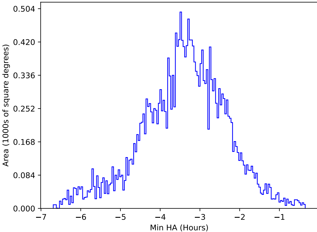
roll_pause_mjdp0_v3.4_10yrs All sky y band: Min HA
