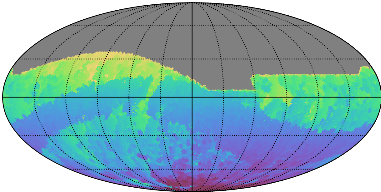
roll_pause_mjdp0_v3.4_10yrs All sky r band: Min HA
