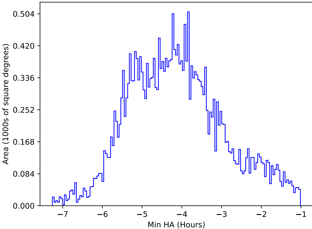
roll_pause_mjdp0_v3.4_10yrs All sky r band: Min HA
