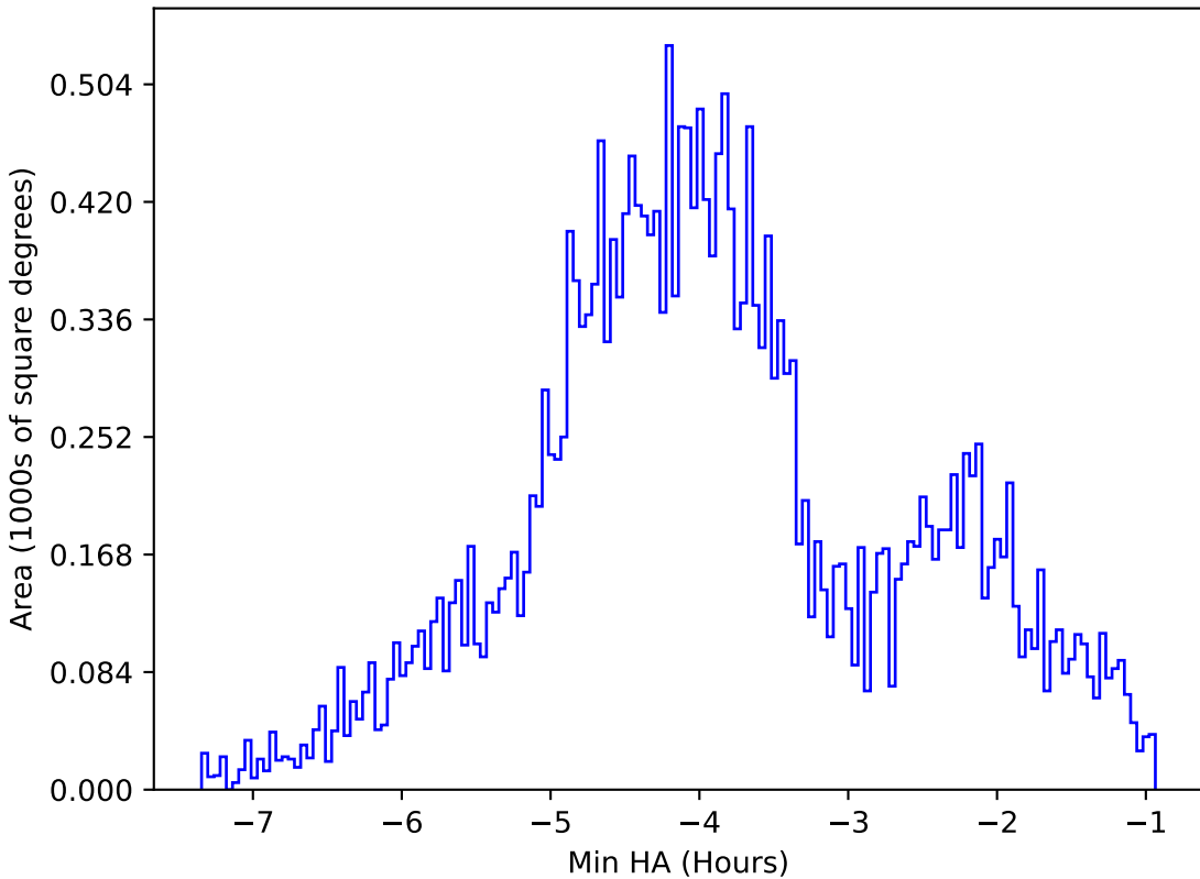
roll_pause_mjdp0_v3.4_10yrs All sky g band: Min HA
