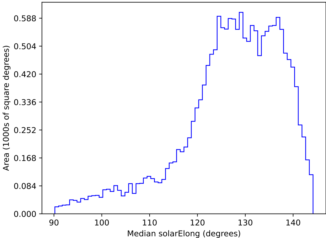
roll_pause_mjdp0_v3.4_10yrs WFD z band: Median solarElong
