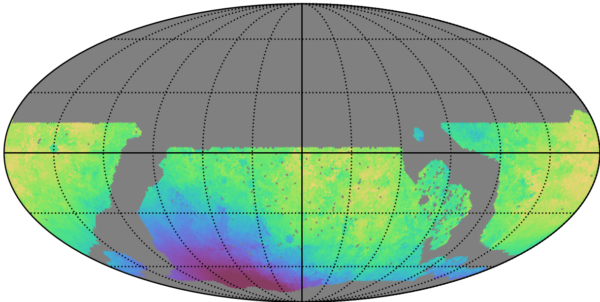
roll_pause_mjdp0_v3.4_10yrs WFD y band: Median solarElong
