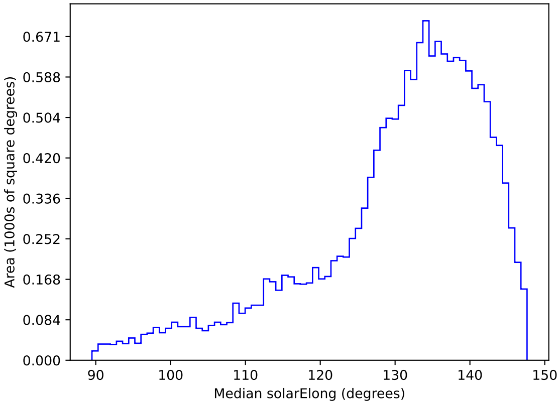
roll_pause_mjdp0_v3.4_10yrs WFD y band: Median solarElong
