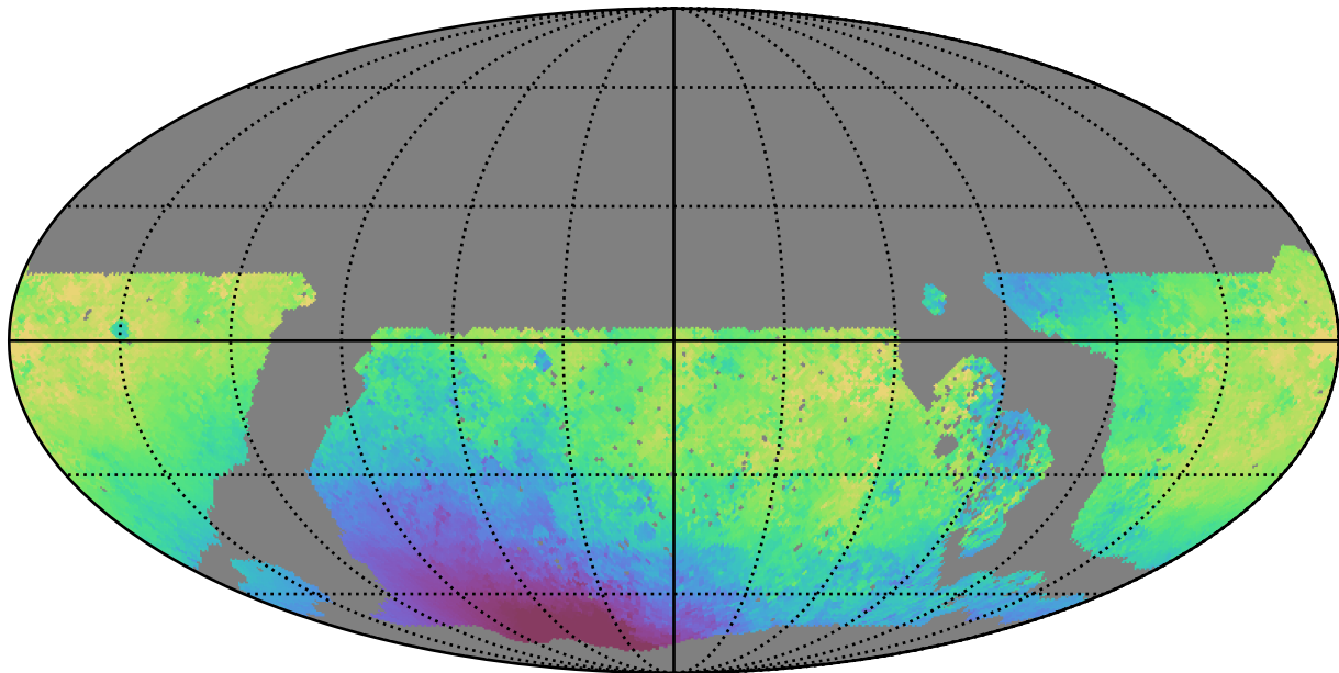
roll_pause_mjdp0_v3.4_10yrs WFD u band: Median solarElong
