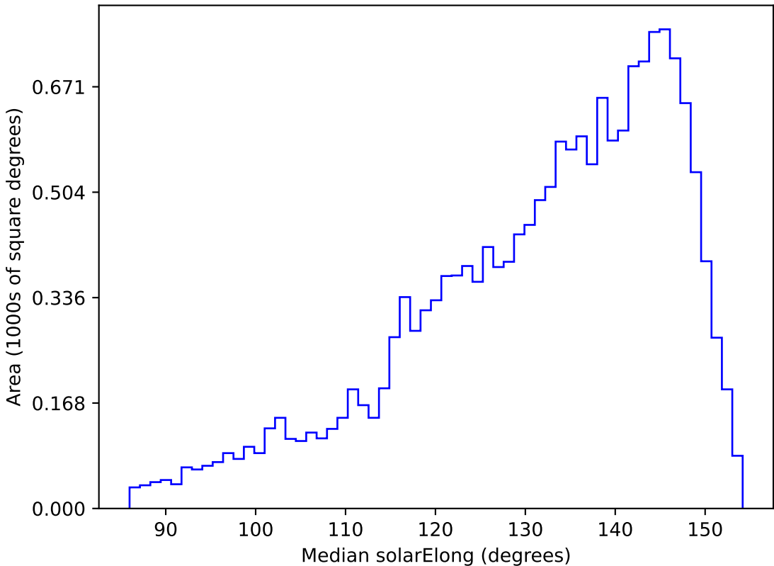
roll_pause_mjdp0_v3.4_10yrs WFD u band: Median solarElong
