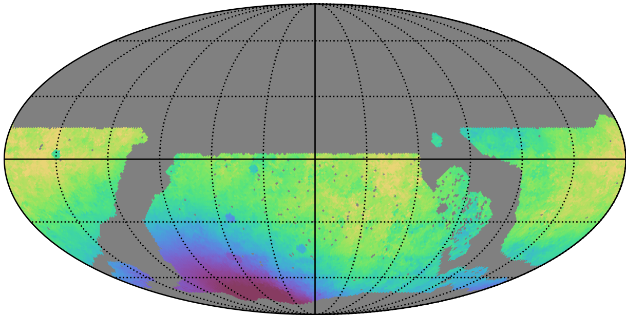
roll_pause_mjdp0_v3.4_10yrs WFD r band: Median solarElong
