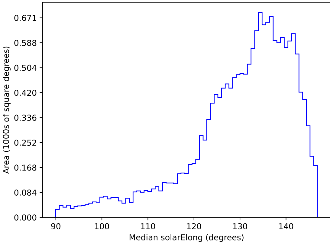
roll_pause_mjdp0_v3.4_10yrs WFD r band: Median solarElong
