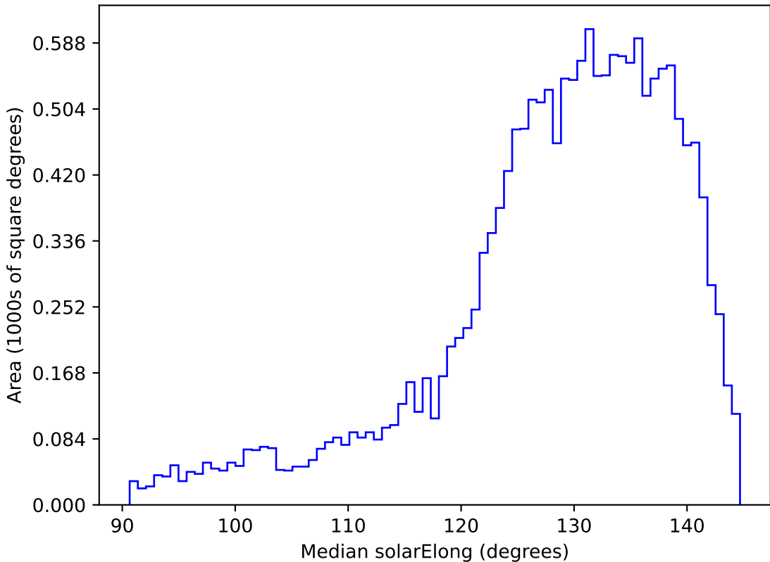
roll_pause_mjdp0_v3.4_10yrs WFD i band: Median solarElong
