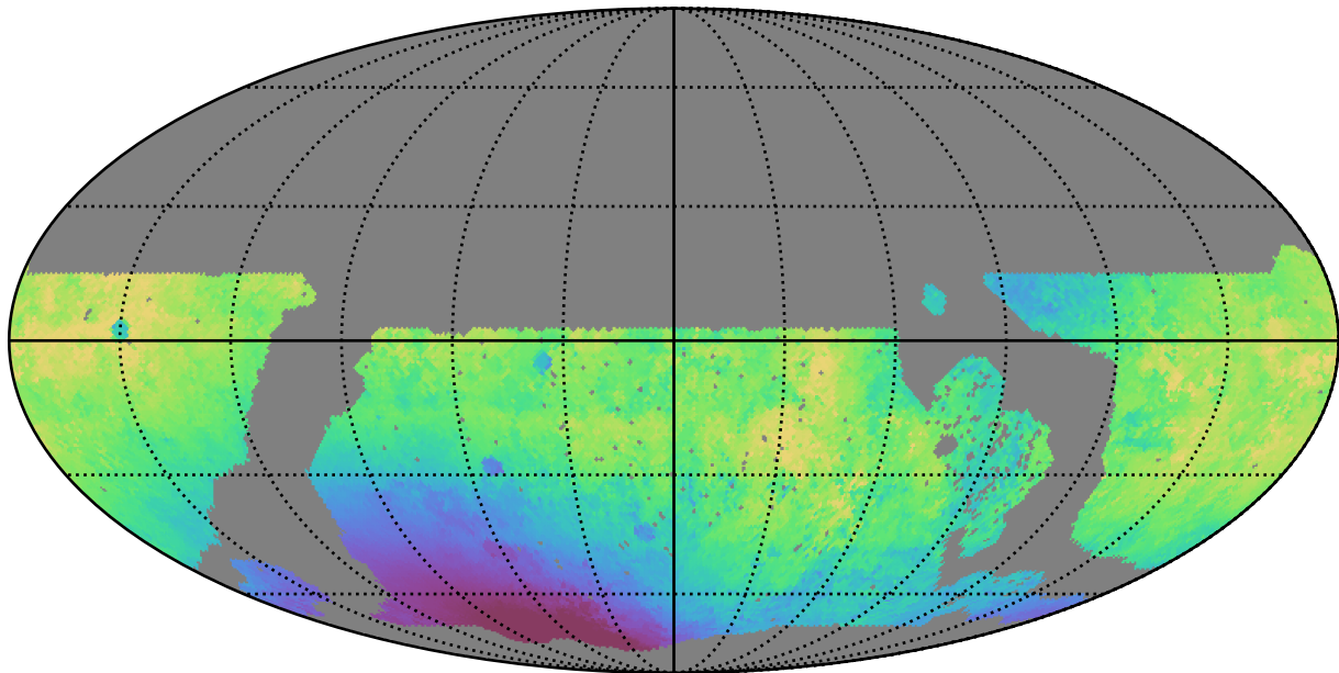
roll_pause_mjdp0_v3.4_10yrs WFD g band: Median solarElong
