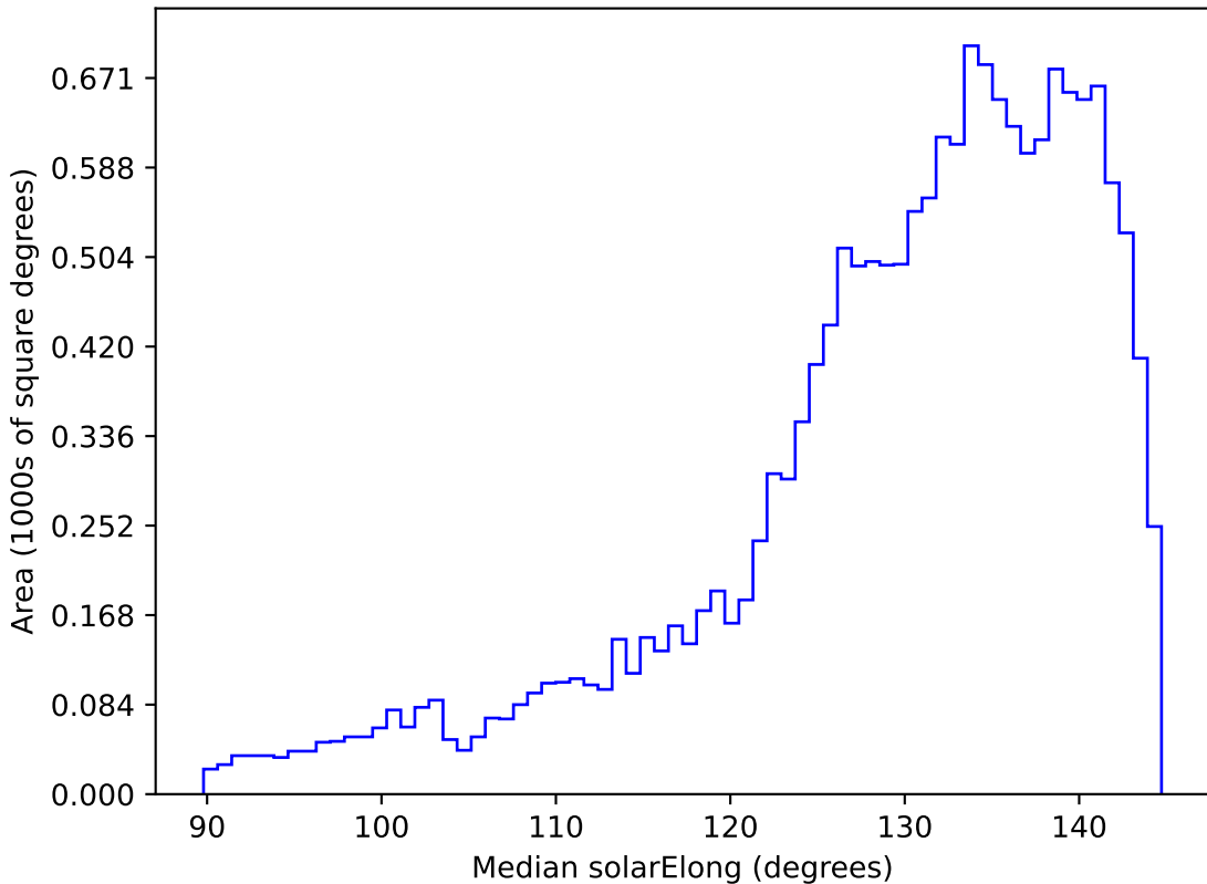
roll_pause_mjdp0_v3.4_10yrs WFD all bands: Median solarElong
