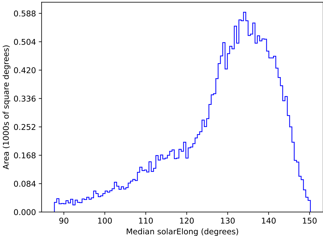
roll_pause_mjdp0_v3.4_10yrs All sky y band: Median solarElong
