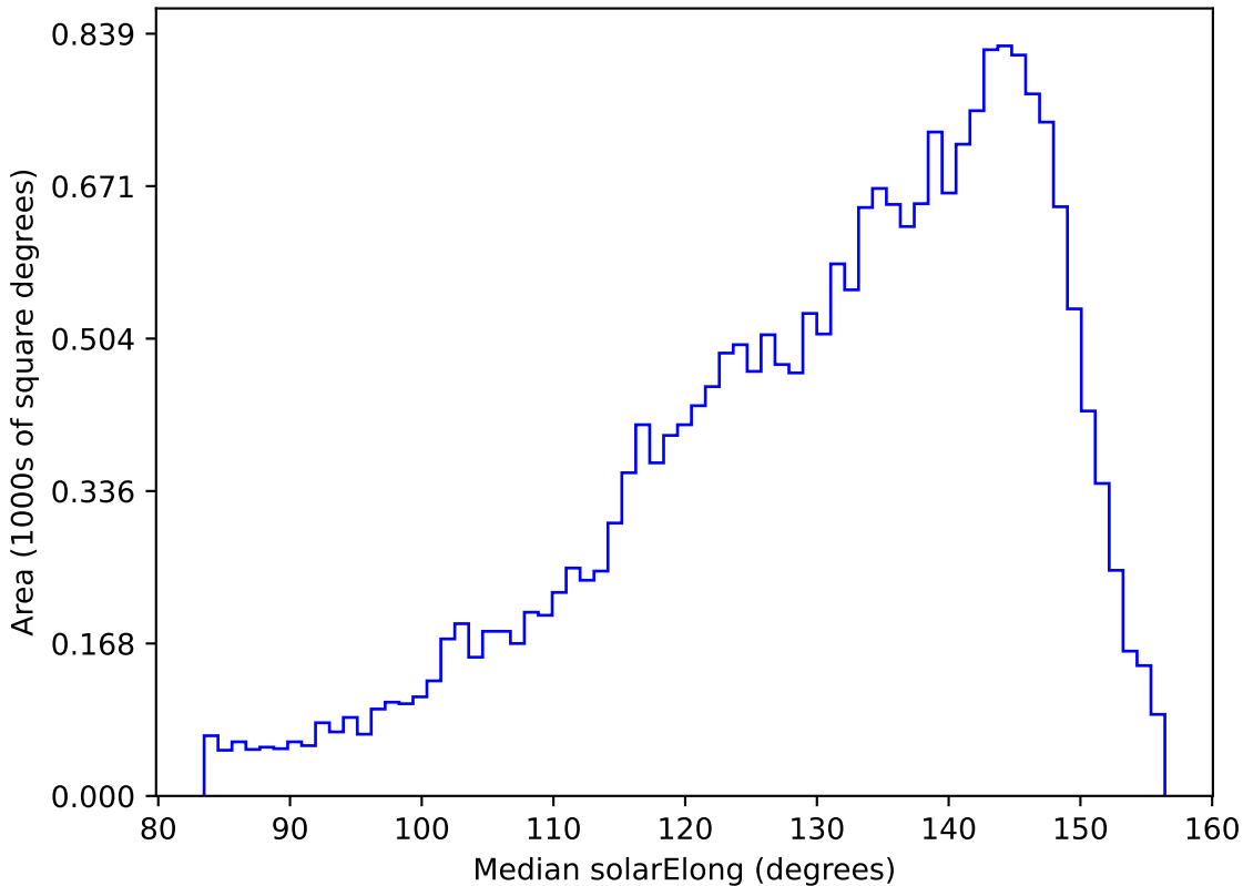
roll_pause_mjdp0_v3.4_10yrs All sky u band: Median solarElong
