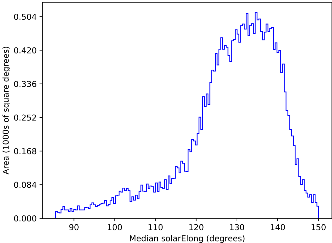
roll_pause_mjdp0_v3.4_10yrs All sky i band: Median solarElong
