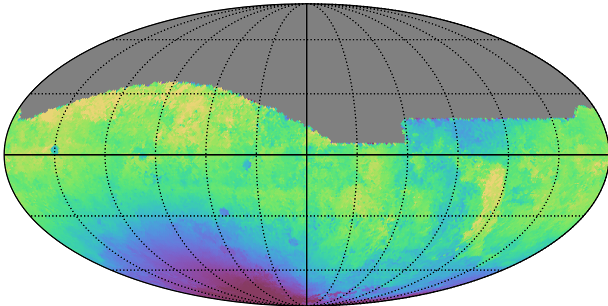
roll_pause_mjdp0_v3.4_10yrs All sky g band: Median solarElong
