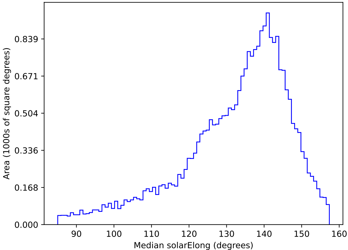
roll_pause_mjdp0_v3.4_10yrs All sky g band: Median solarElong
