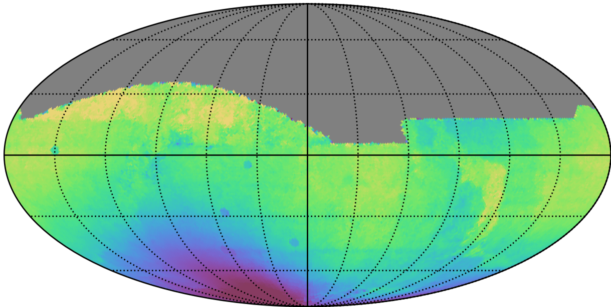
roll_pause_mjdp0_v3.4_10yrs All sky all bands: Median solarElong
