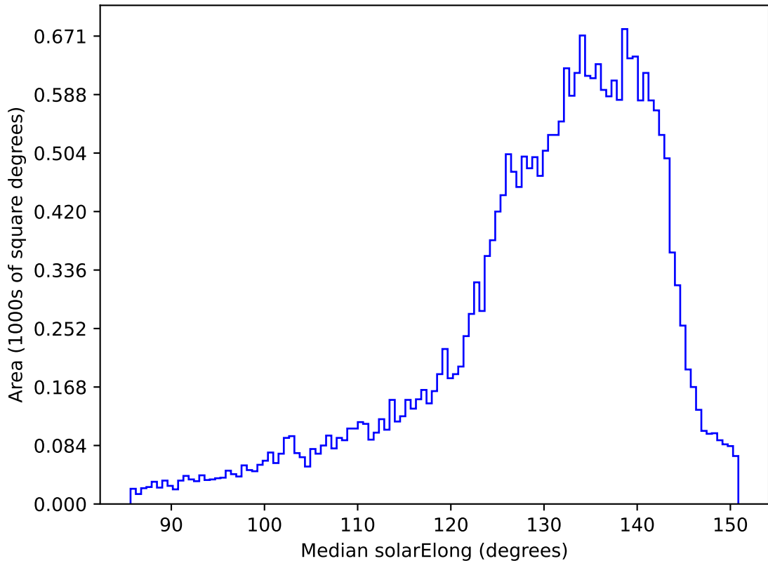
roll_pause_mjdp0_v3.4_10yrs All sky all bands: Median solarElong
