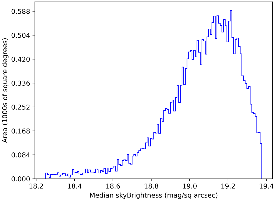
roll_pause_mjdp0_v3.4_10yrs Yr 1 z band: Median skyBrightness
