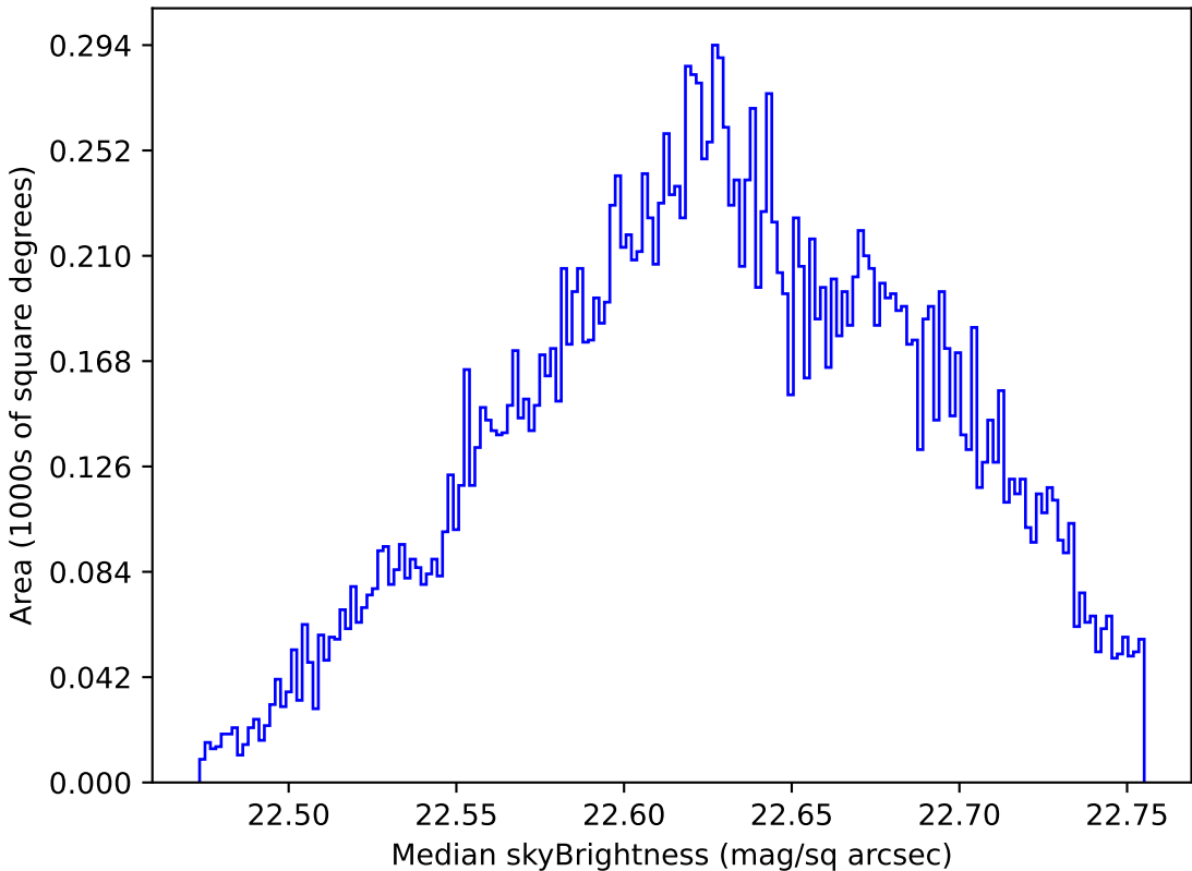
roll_pause_mjdp0_v3.4_10yrs Yr 1 u band: Median skyBrightness
