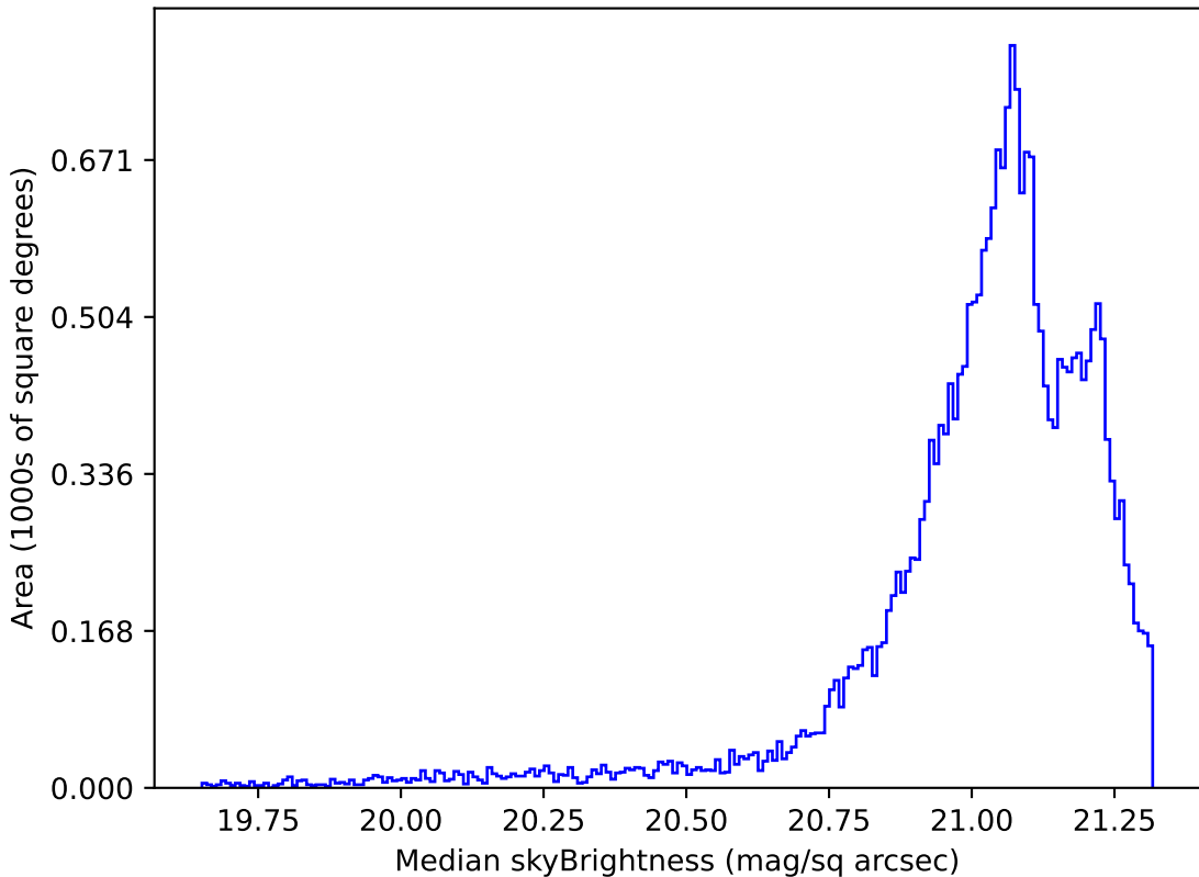
roll_pause_mjdp0_v3.4_10yrs Yr 1 r band: Median skyBrightness
