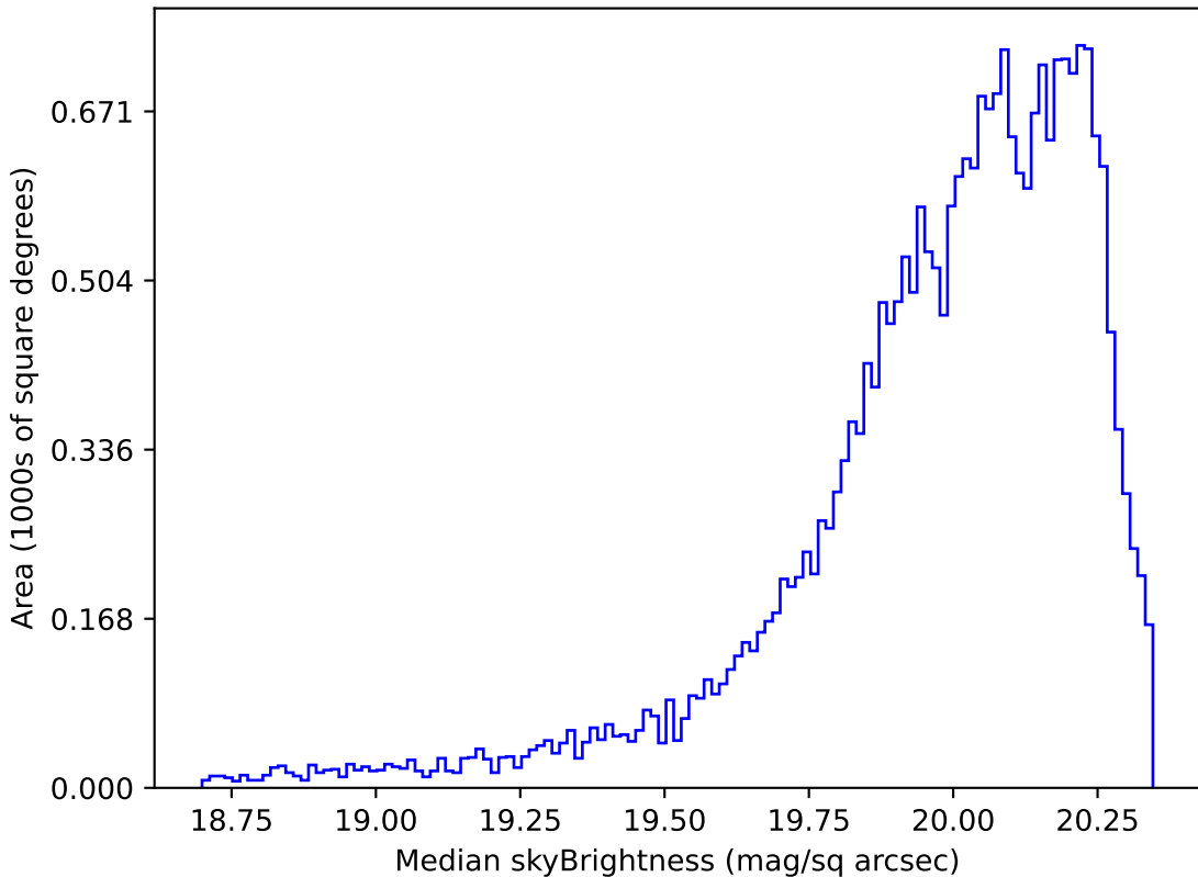
roll_pause_mjdp0_v3.4_10yrs Yr 1 i band: Median skyBrightness
