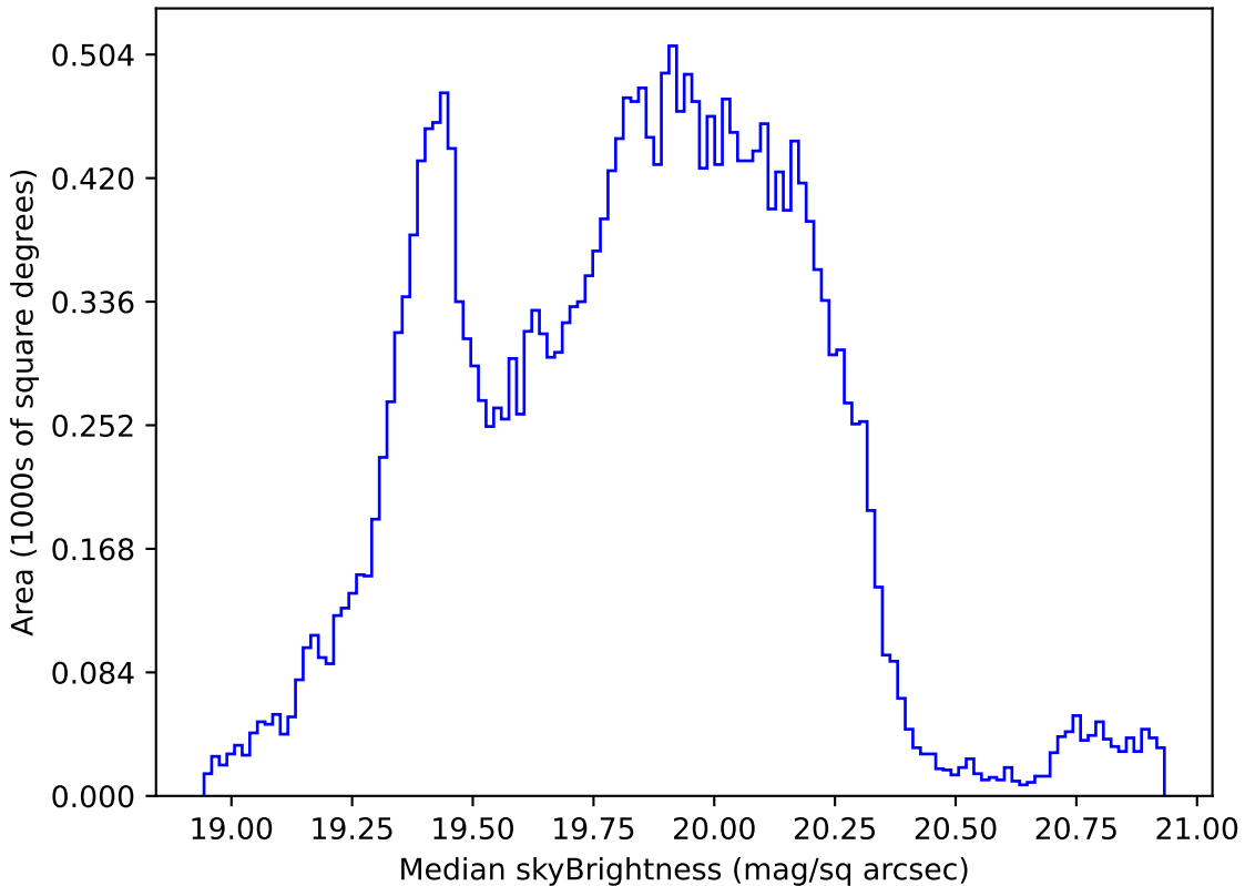
roll_pause_mjdp0_v3.4_10yrs Yr 1 all bands: Median skyBrightness
