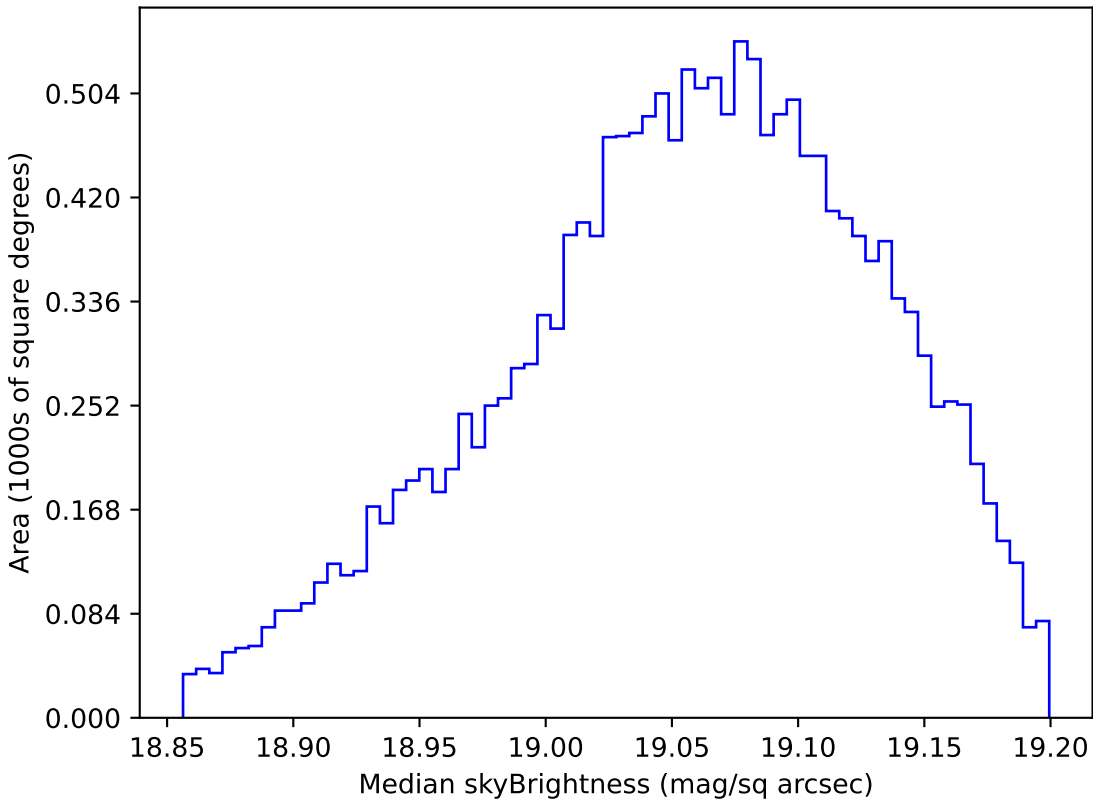
roll_pause_mjdp0_v3.4_10yrs WFD z band: Median skyBrightness
