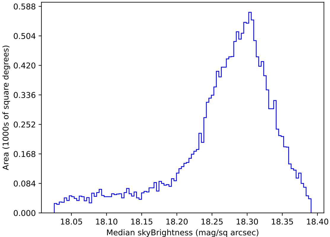
roll_pause_mjdp0_v3.4_10yrs WFD y band: Median skyBrightness
