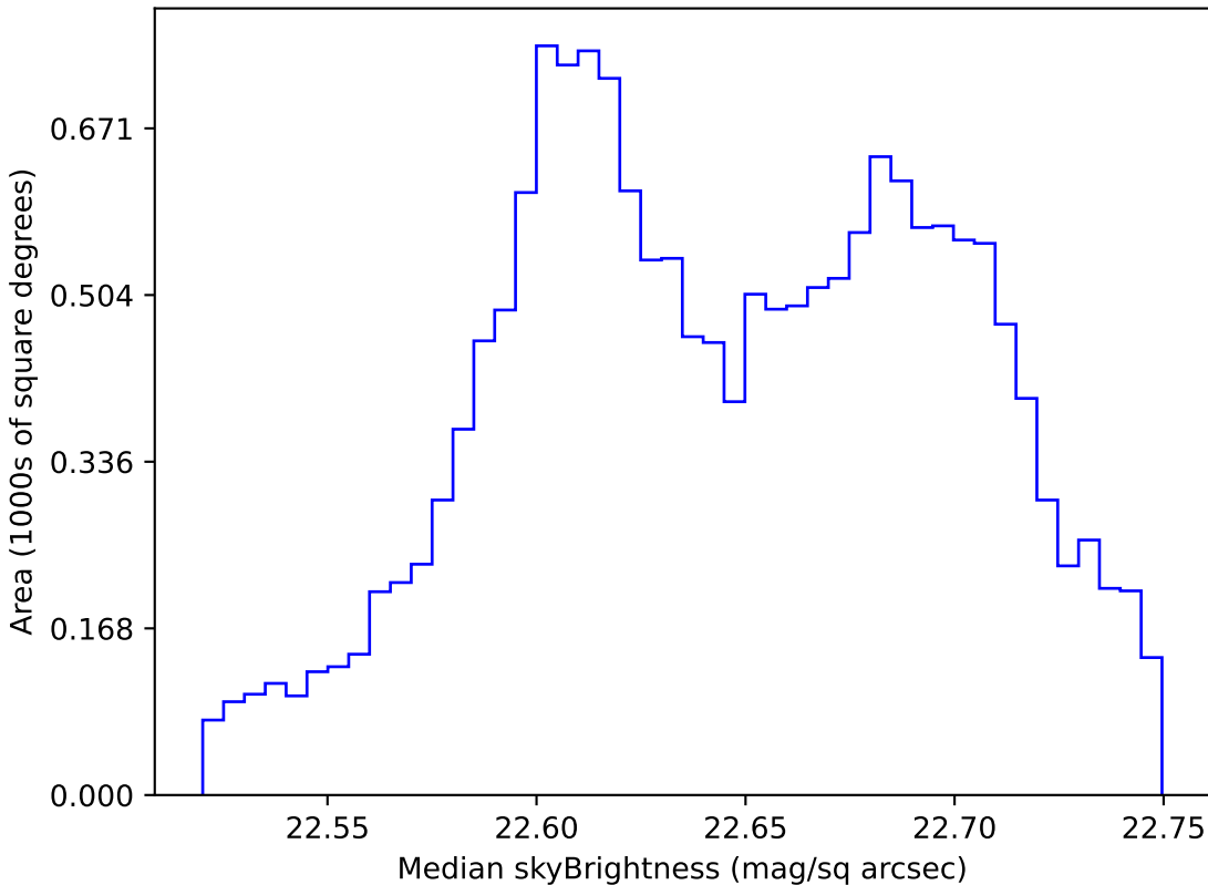
roll_pause_mjdp0_v3.4_10yrs WFD u band: Median skyBrightness
