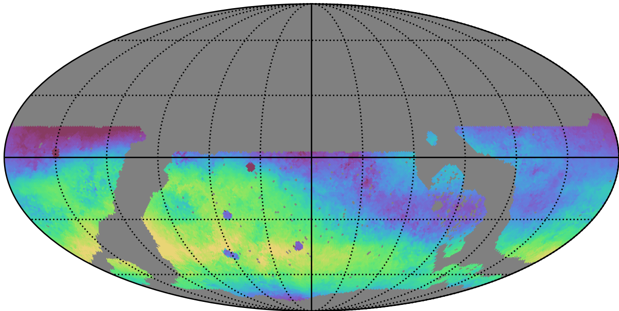
roll_pause_mjdp0_v3.4_10yrs WFD r band: Median skyBrightness
