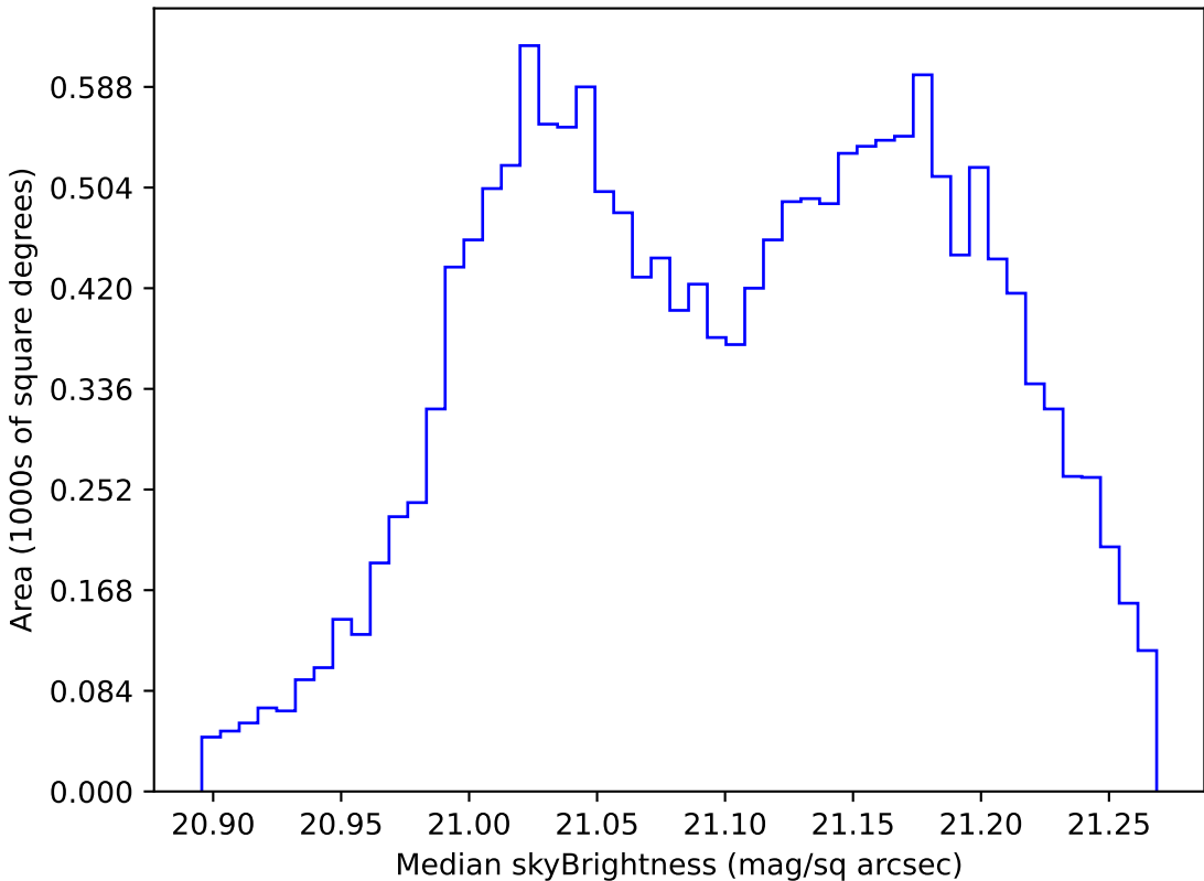
roll_pause_mjdp0_v3.4_10yrs WFD r band: Median skyBrightness
