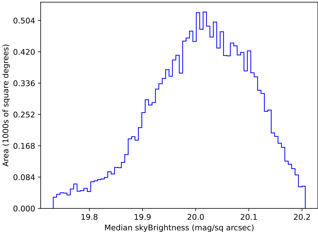
roll_pause_mjdp0_v3.4_10yrs WFD i band: Median skyBrightness
