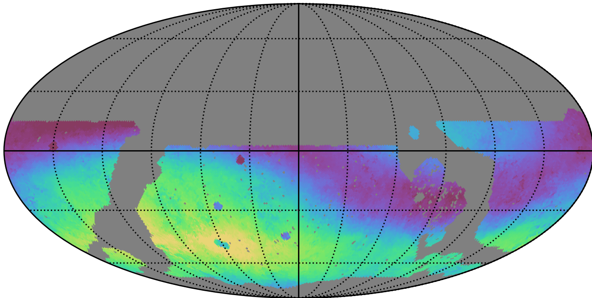
roll_pause_mjdp0_v3.4_10yrs WFD g band: Median skyBrightness
