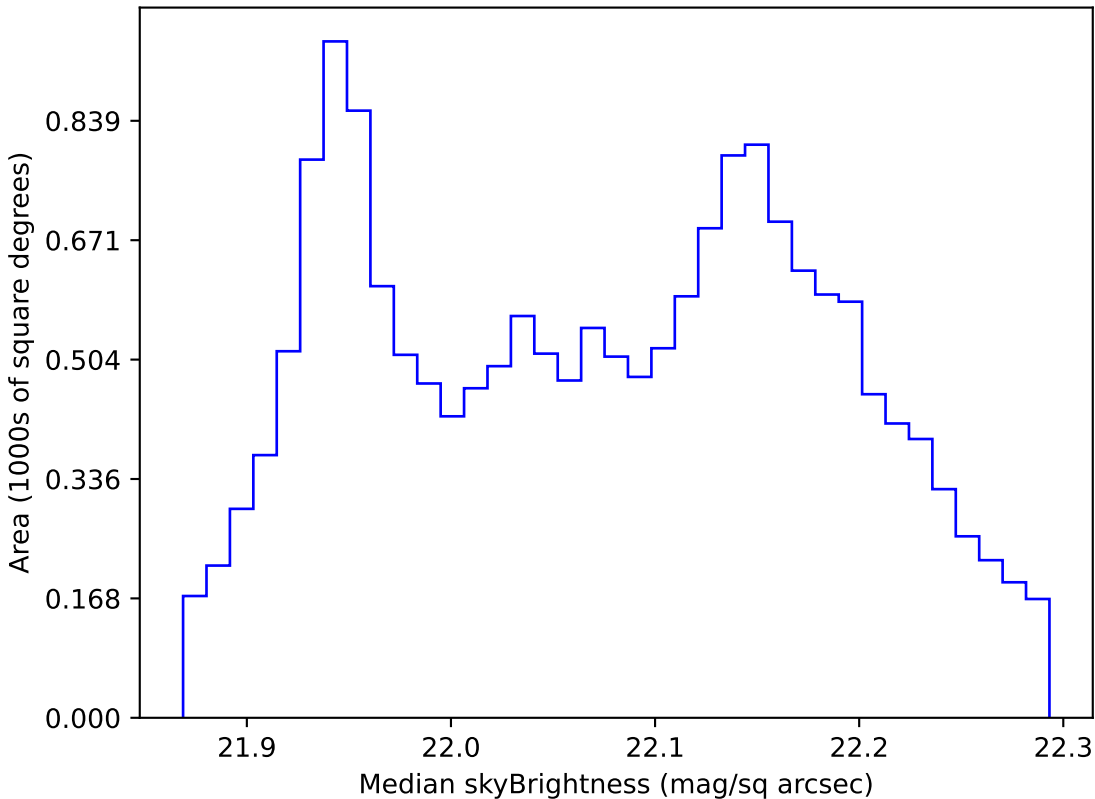
roll_pause_mjdp0_v3.4_10yrs WFD g band: Median skyBrightness
