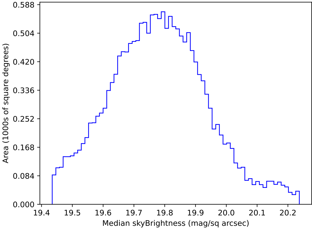
roll_pause_mjdp0_v3.4_10yrs WFD all bands: Median skyBrightness
