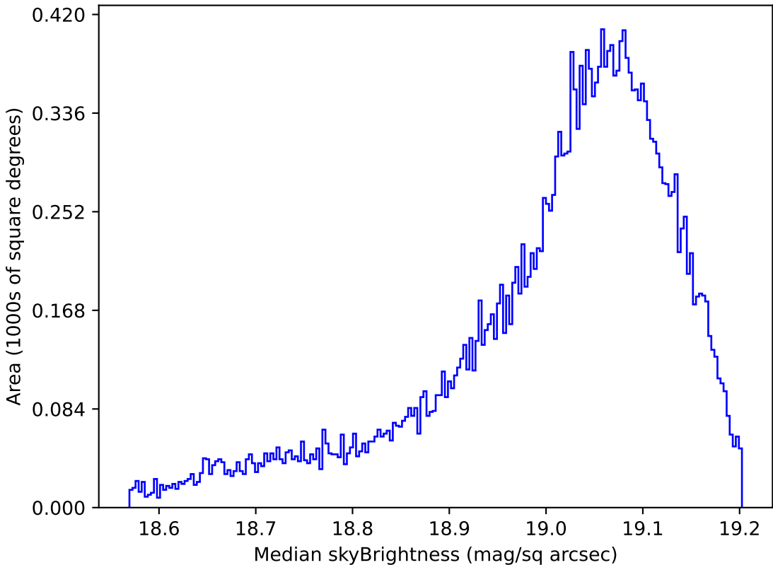
roll_pause_mjdp0_v3.4_10yrs All sky z band: Median skyBrightness
