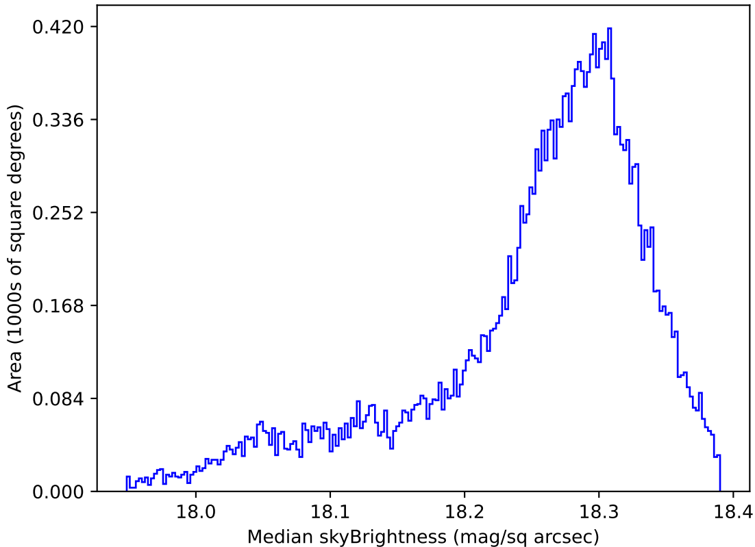
roll_pause_mjdp0_v3.4_10yrs All sky y band: Median skyBrightness
