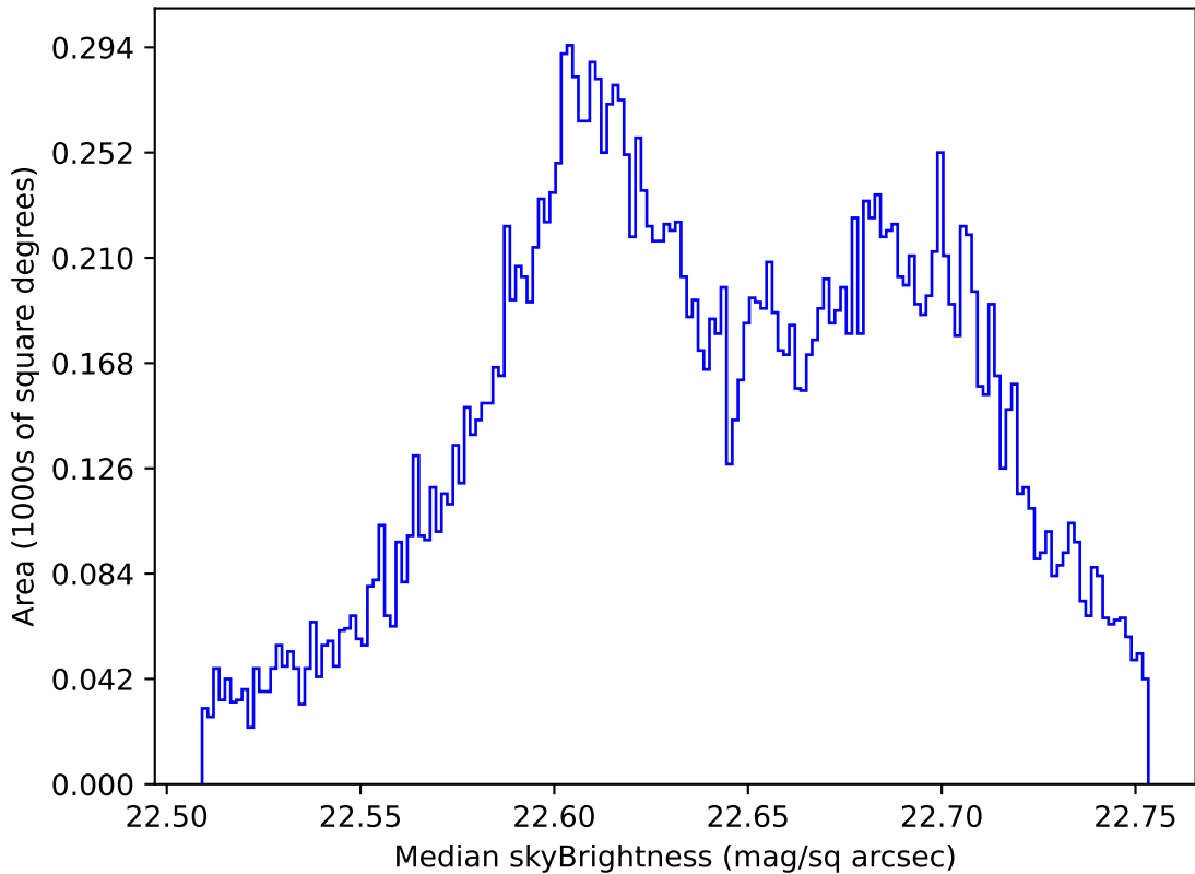
roll_pause_mjdp0_v3.4_10yrs All sky u band: Median skyBrightness
