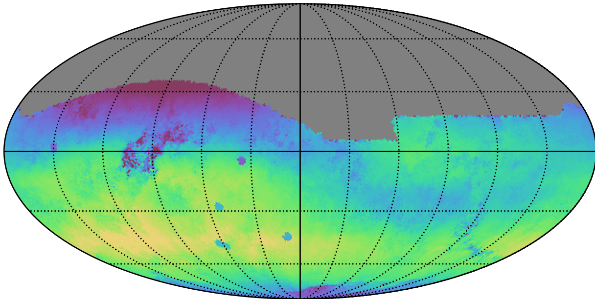
roll_pause_mjdp0_v3.4_10yrs All sky r band: Median skyBrightness
