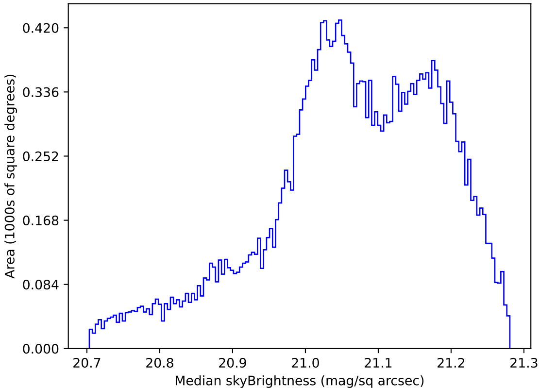
roll_pause_mjdp0_v3.4_10yrs All sky r band: Median skyBrightness
