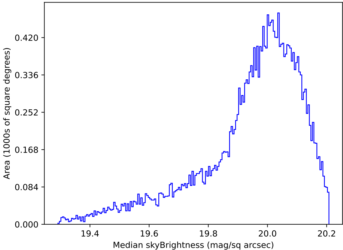
roll_pause_mjdp0_v3.4_10yrs All sky i band: Median skyBrightness
